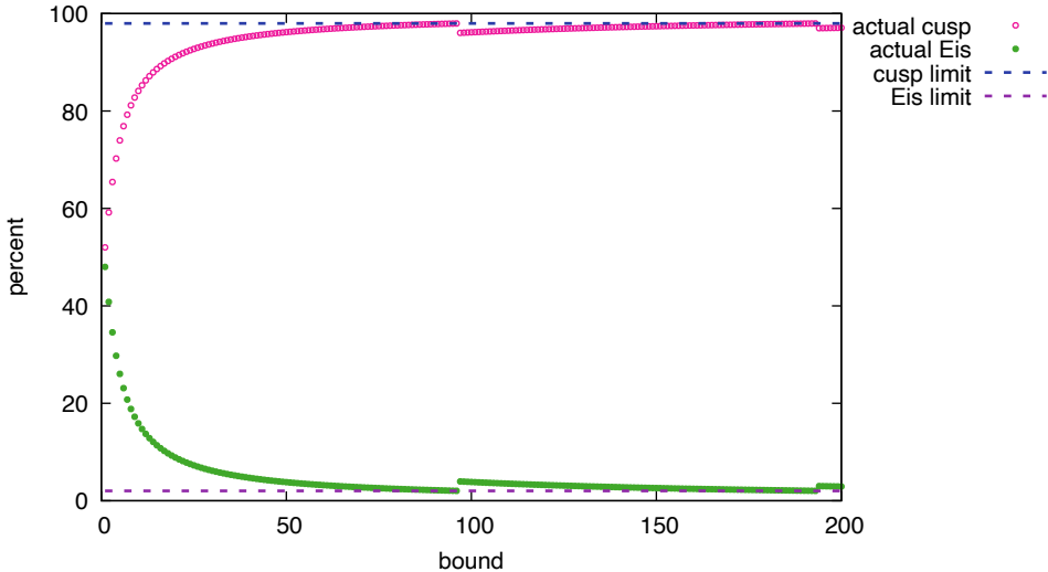
Cuspidal and Eisenstein Percentages for N = 97
