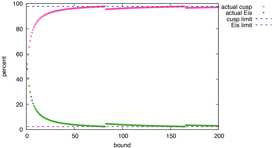
Cuspidal and Eisenstein Percentages for N = 83
