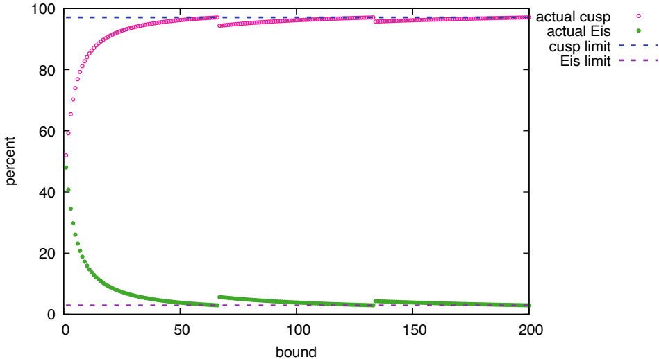
Cuspidal and Eisenstein Percentages for N = 67
