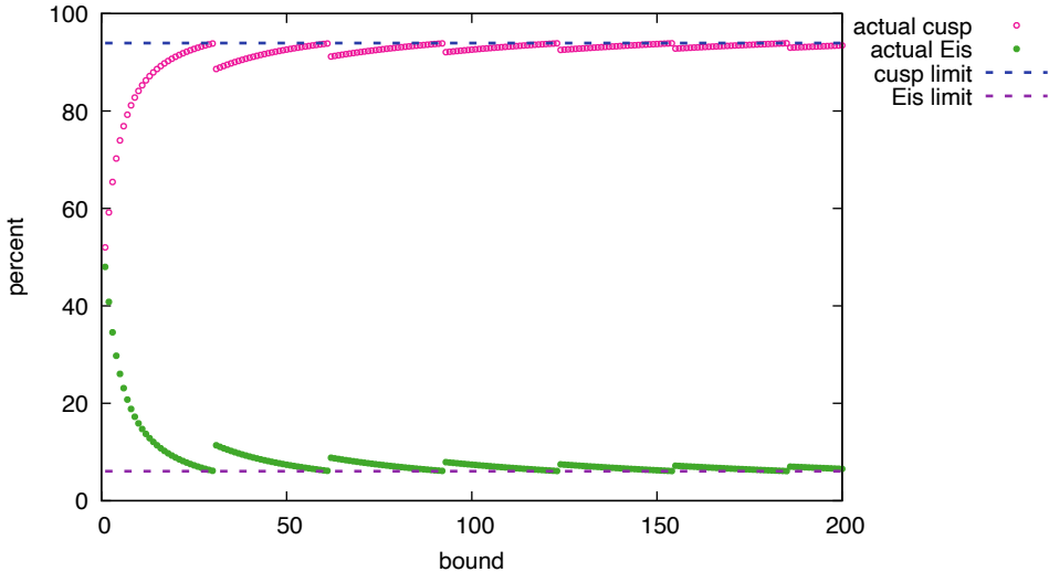
Cuspidal and Eisenstein Percentages for N = 31
